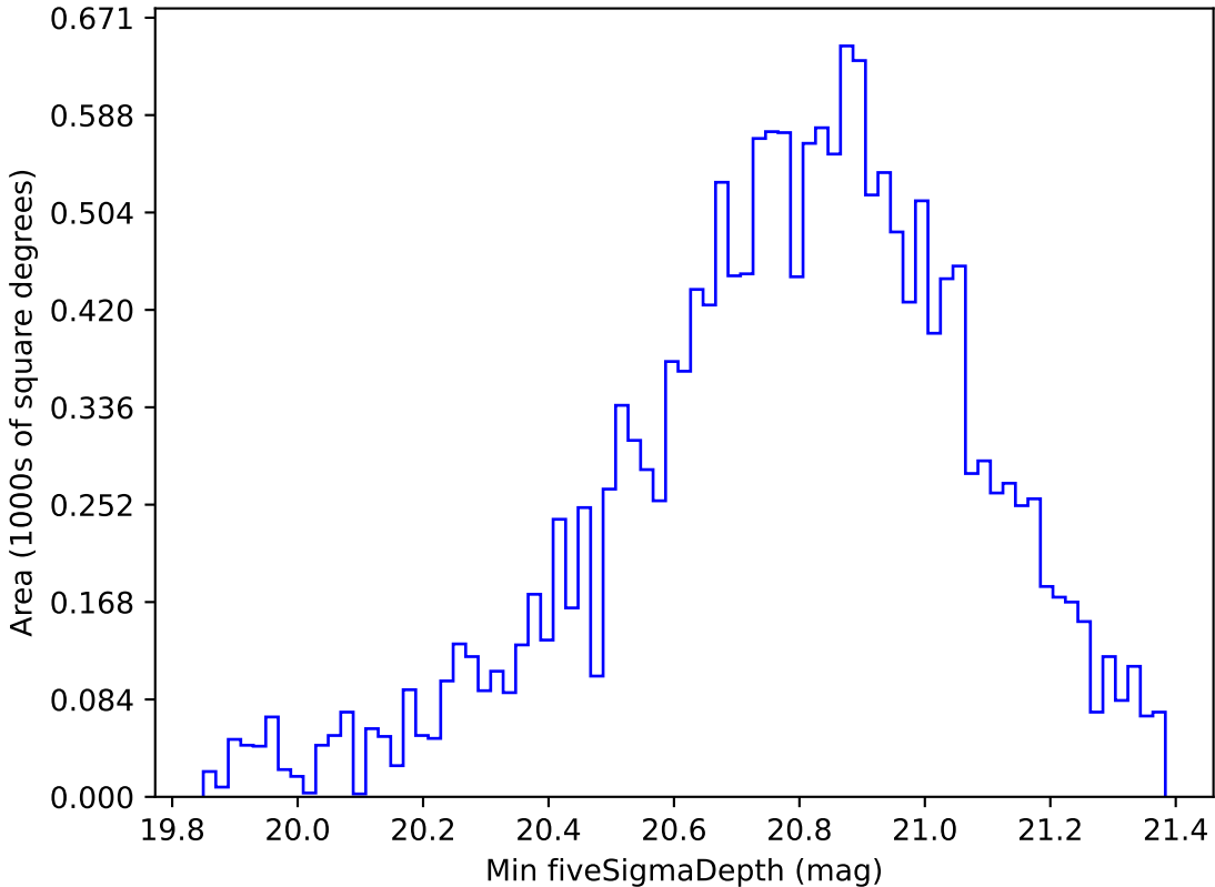
ddf_loaded_fl1_v3.4_10yrs WFD all bands: Min fiveSigmaDepth
