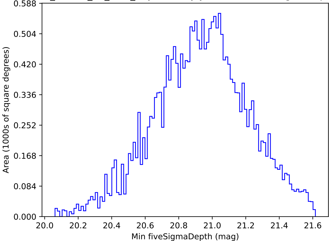
ddf_loaded_fl1_v3.4_10yrs All sky y band: Min fiveSigmaDepth
