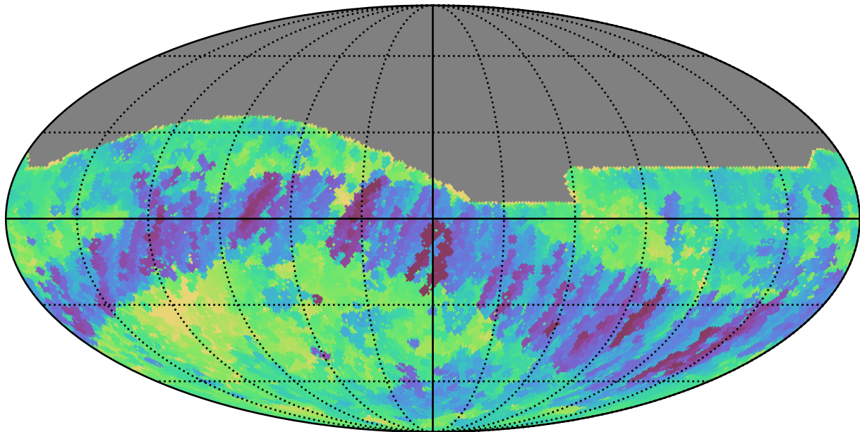
ddf_loaded_fl1_v3.4_10yrs All sky r band: Min fiveSigmaDepth
