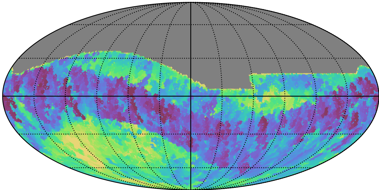
ddf_loaded_fl1_v3.4_10yrs All sky i band: Min fiveSigmaDepth
