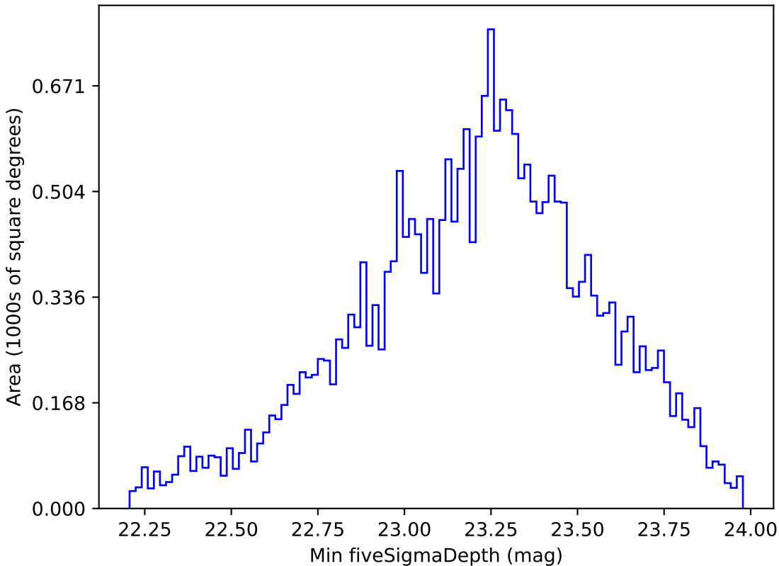
ddf_loaded_fl1_v3.4_10yrs All sky g band: Min fiveSigmaDepth
