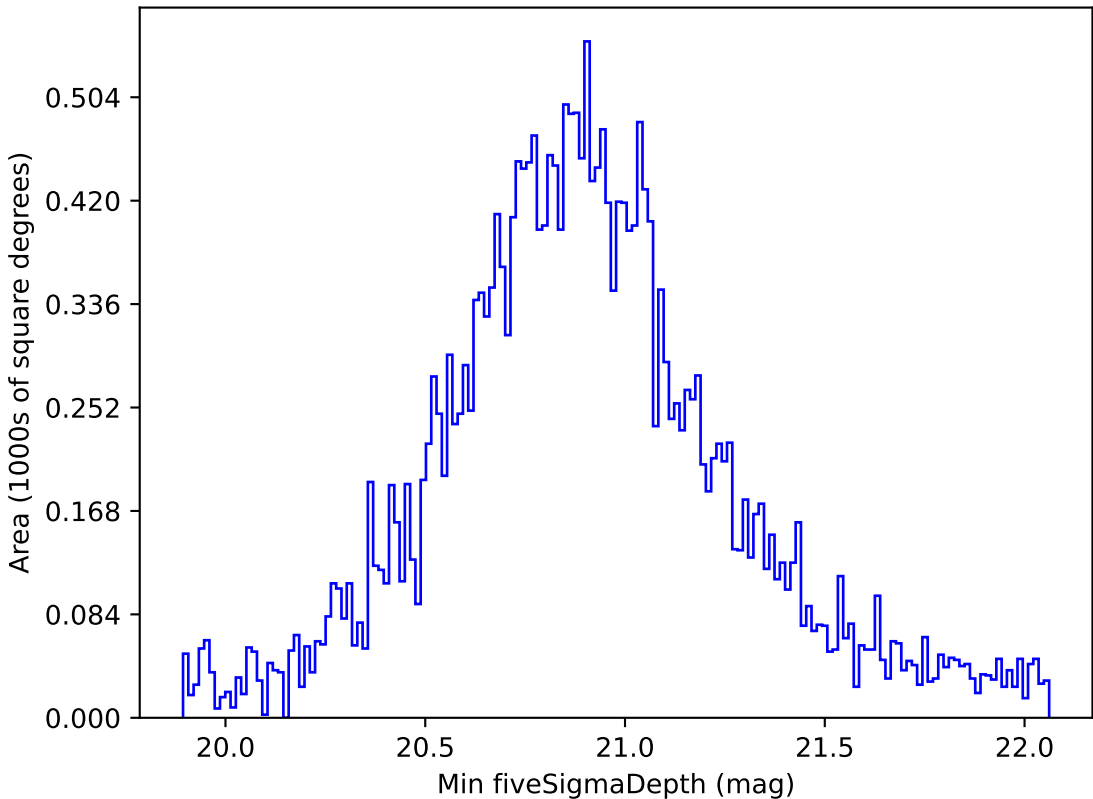
ddf_loaded_fl1_v3.4_10yrs All sky all bands: Min fiveSigmaDepth
