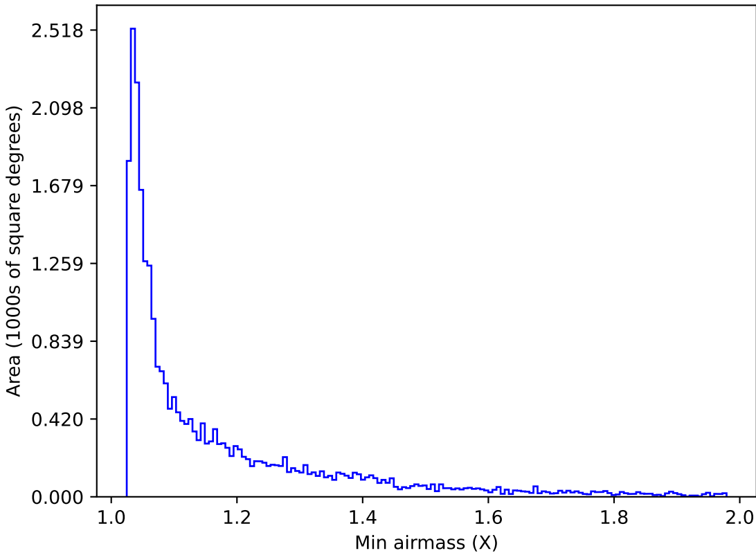
ddf_loaded_fl1_v3.4_10yrs Yr 1 z band: Min airmass
