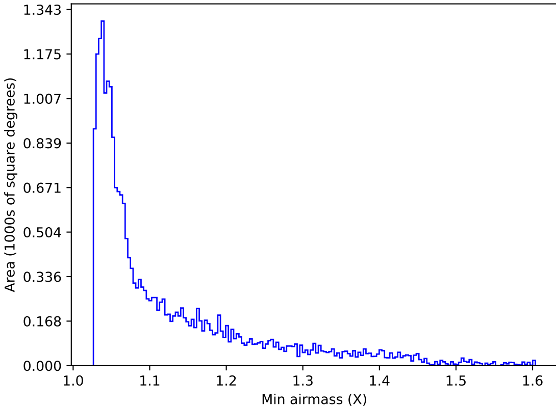
ddf_loaded_fl1_v3.4_10yrs Yr 1 y band: Min airmass
