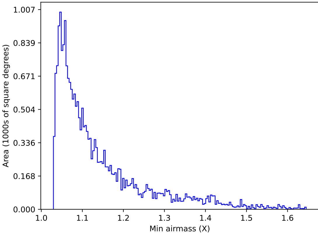
ddf_loaded_fl1_v3.4_10yrs Yr 1 u band: Min airmass
