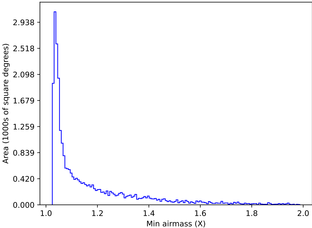
ddf_loaded_fl1_v3.4_10yrs Yr 1 r band: Min airmass
