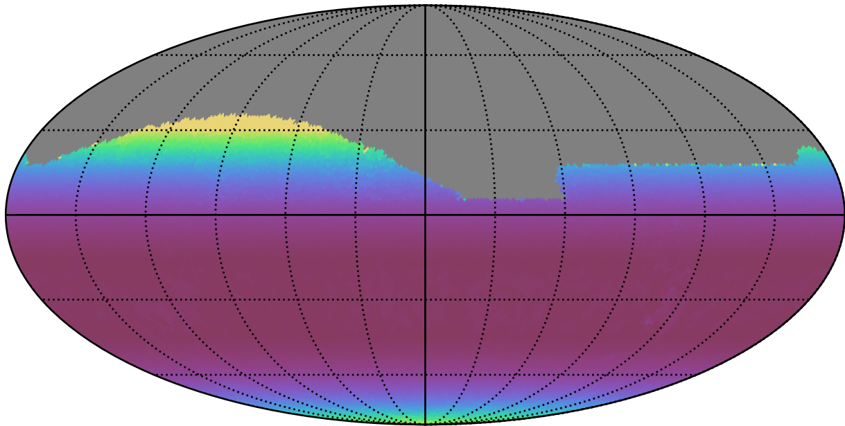
ddf_loaded_fl1_v3.4_10yrs Yr 1 all bands: Min airmass
