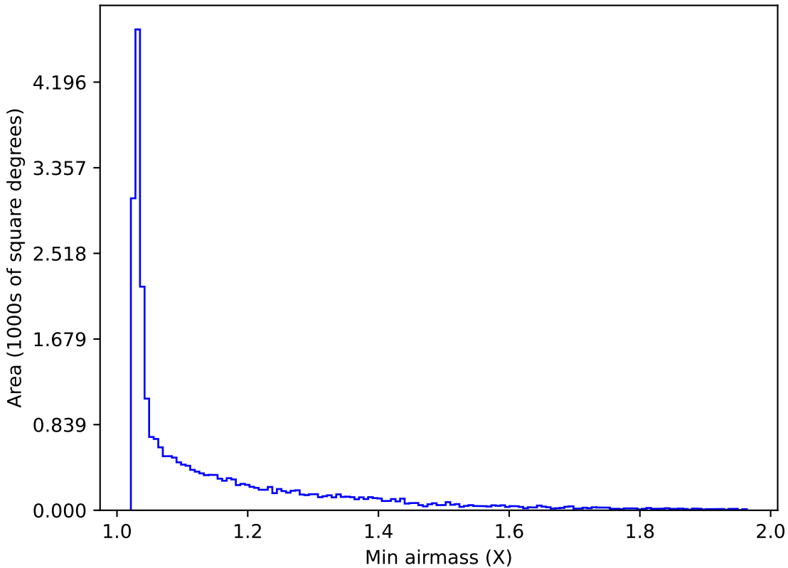
ddf_loaded_fl1_v3.4_10yrs Yr 1 all bands: Min airmass
