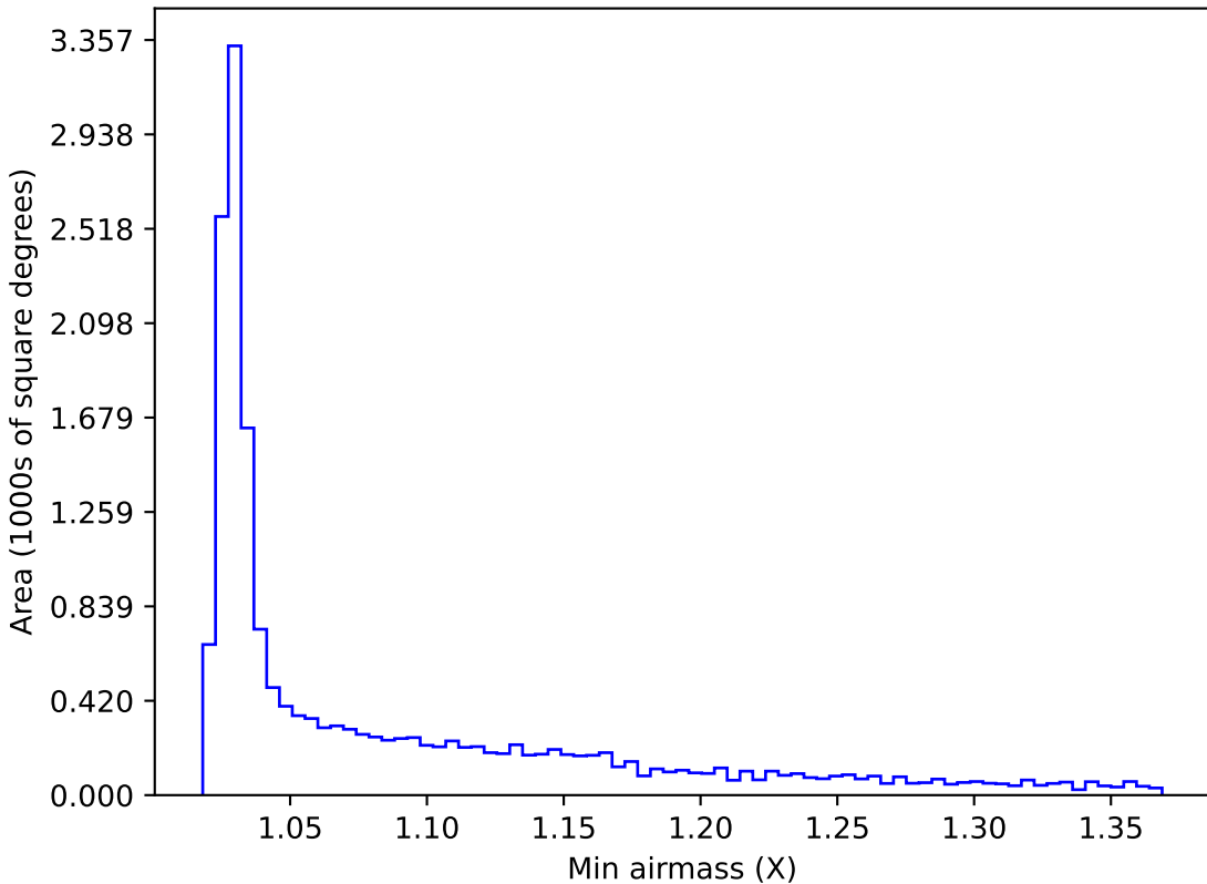
ddf_loaded_fl1_v3.4_10yrs WFD z band: Min airmass
