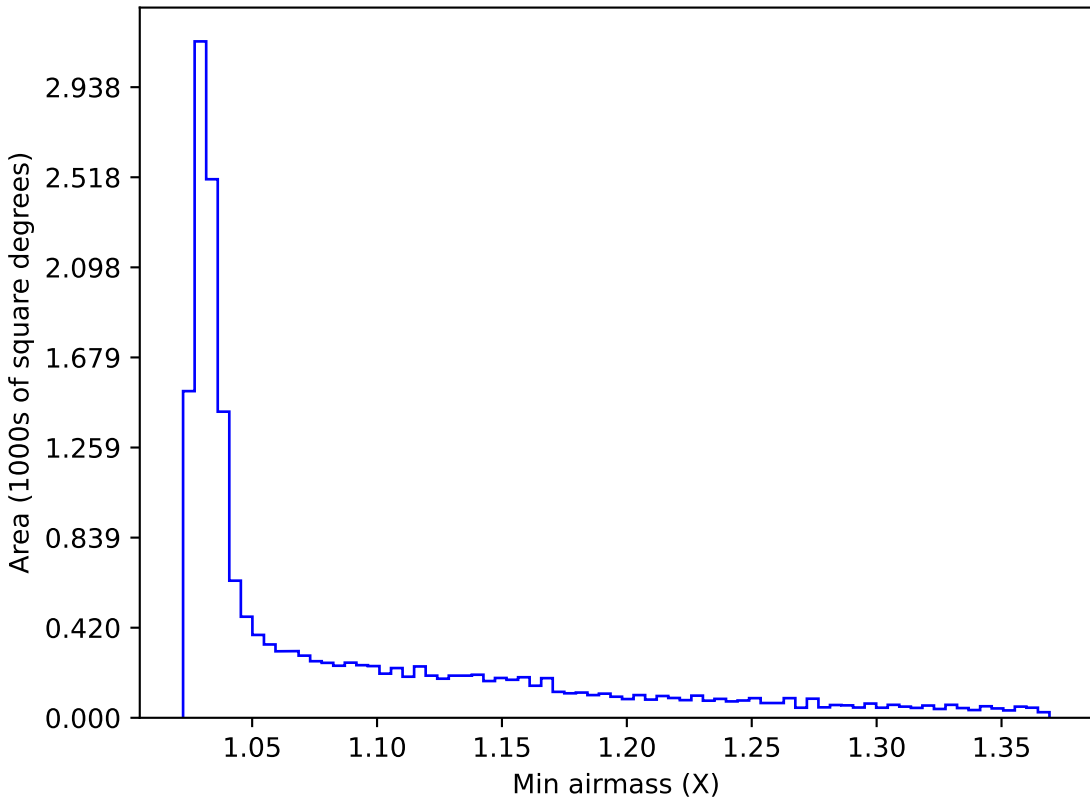
ddf_loaded_fl1_v3.4_10yrs WFD y band: Min airmass
