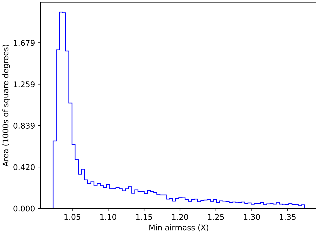
ddf_loaded_fl1_v3.4_10yrs WFD u band: Min airmass
