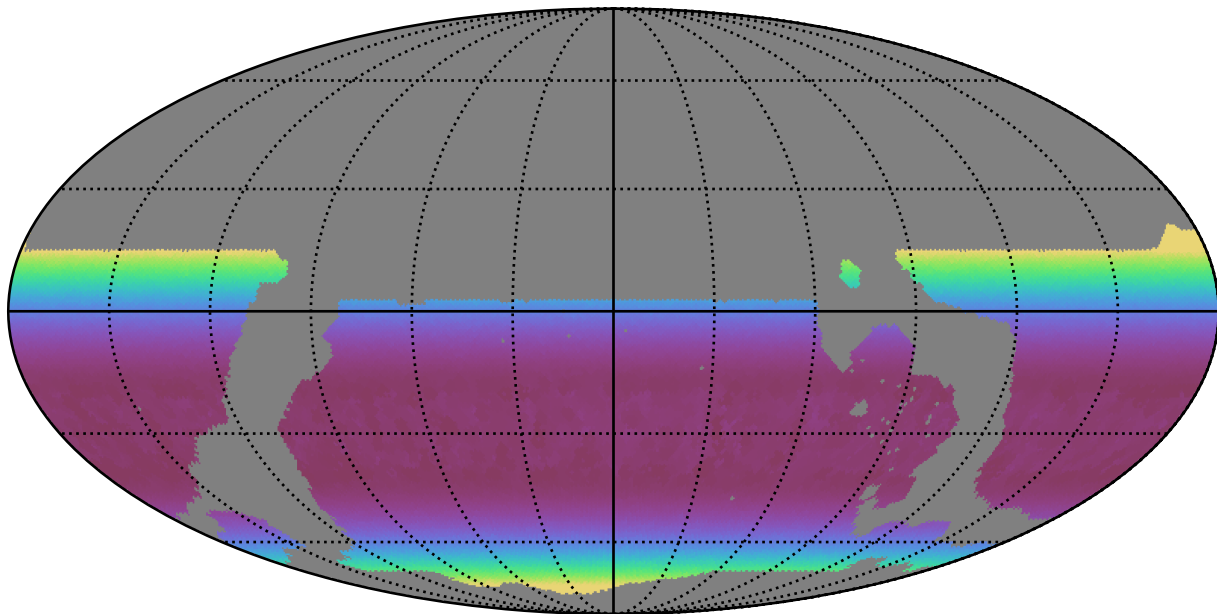
ddf_loaded_fl1_v3.4_10yrs WFD r band: Min airmass
