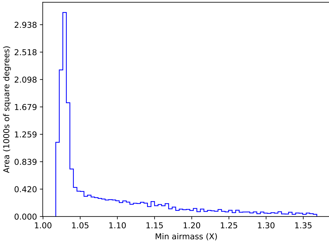
ddf_loaded_fl1_v3.4_10yrs WFD r band: Min airmass
