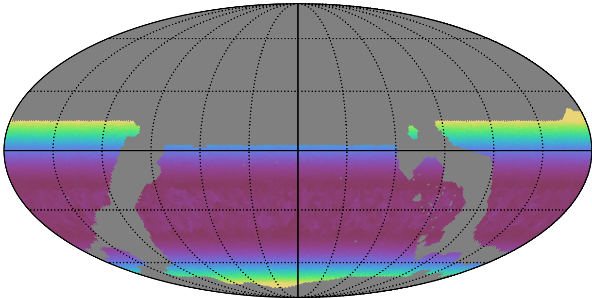
ddf_loaded_fl1_v3.4_10yrs WFD g band: Min airmass
