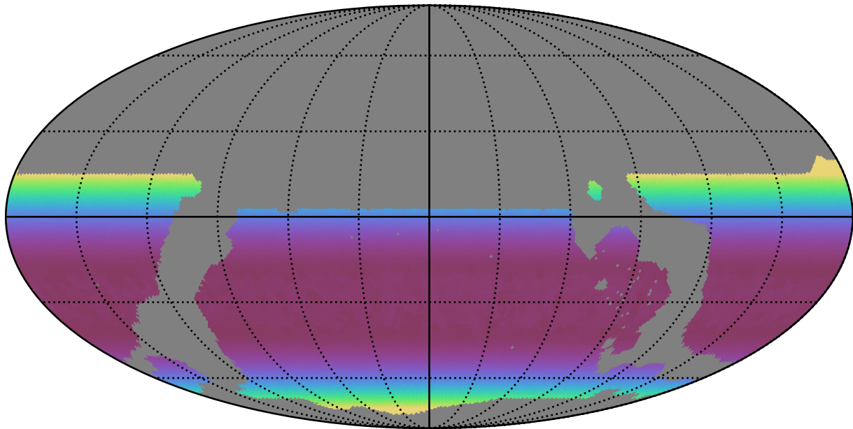
ddf_loaded_fl1_v3.4_10yrs WFD all bands: Min airmass
