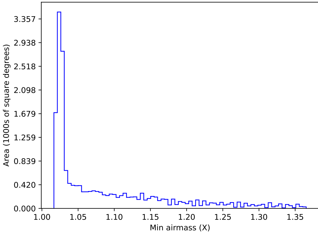
ddf_loaded_fl1_v3.4_10yrs WFD all bands: Min airmass
