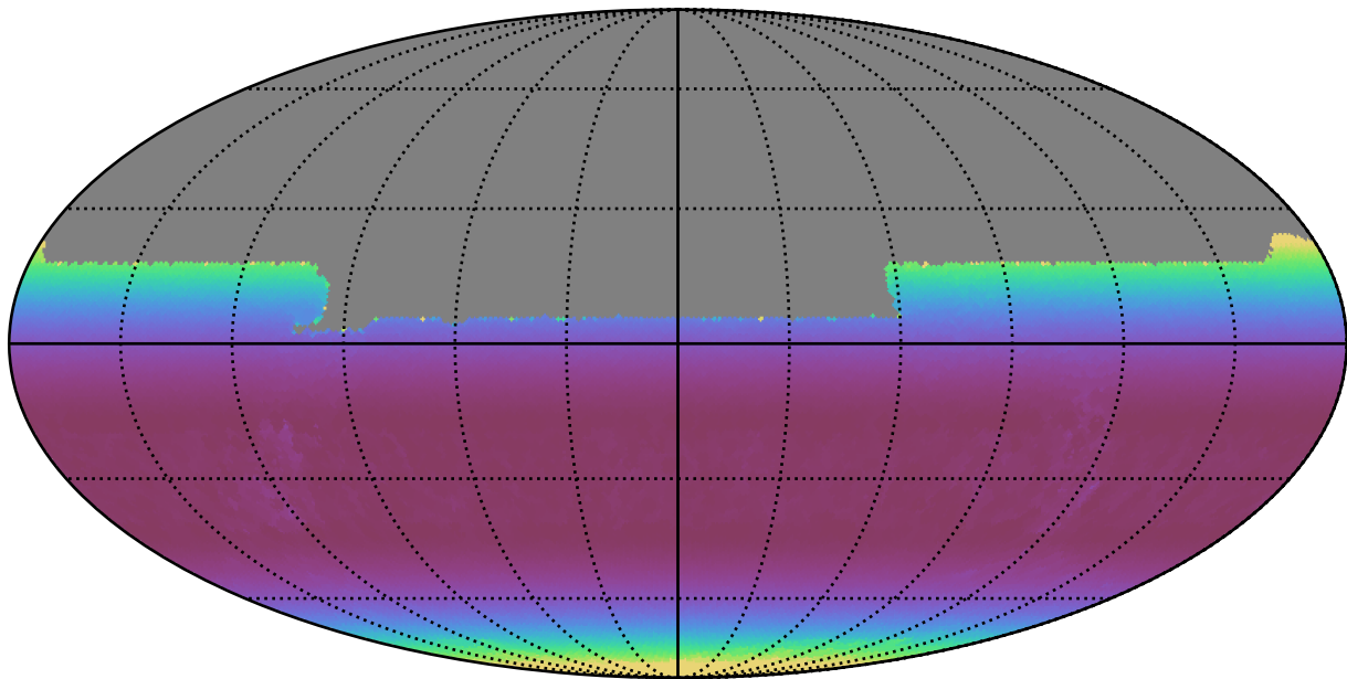
ddf_loaded_fl1_v3.4_10yrs All sky y band: Min airmass
