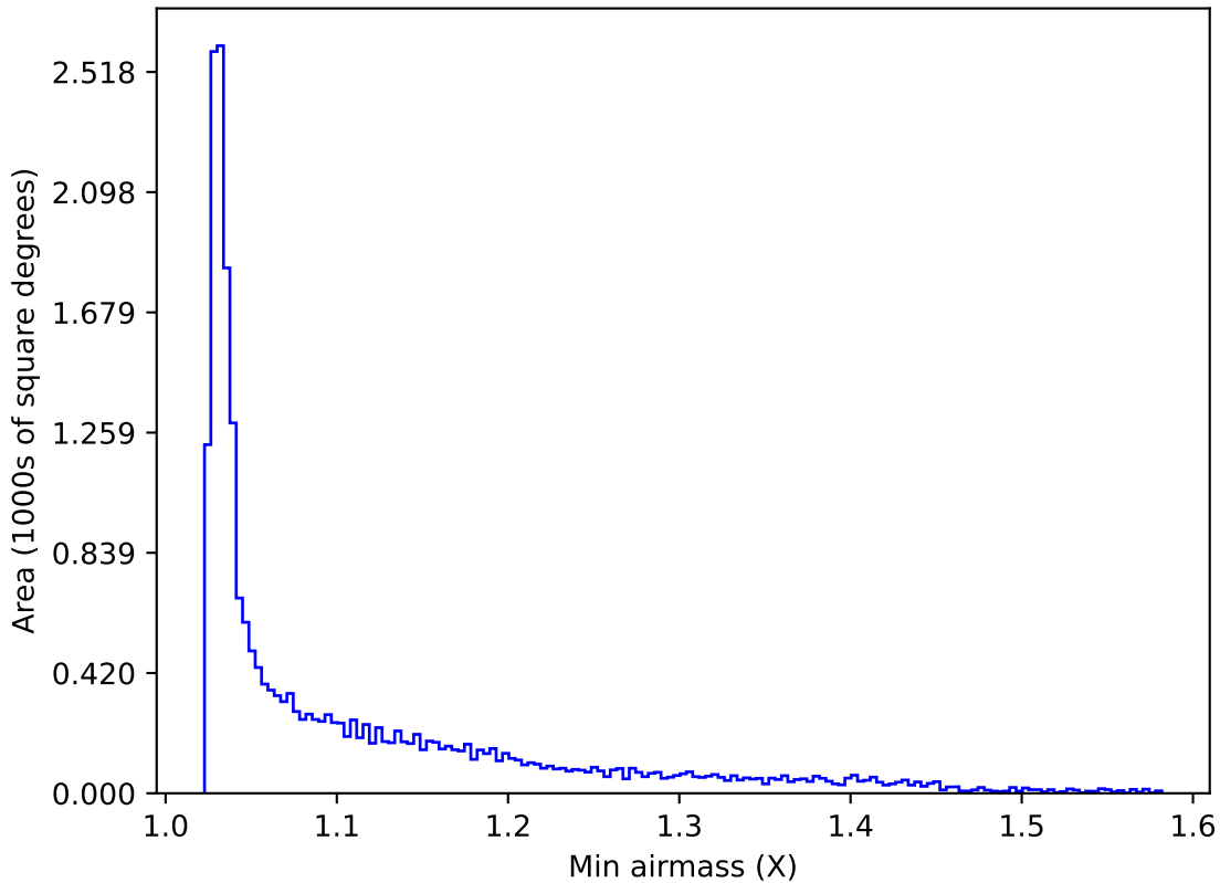
ddf_loaded_fl1_v3.4_10yrs All sky y band: Min airmass
