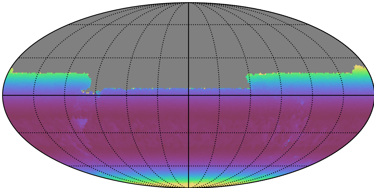
ddf_loaded_fl1_v3.4_10yrs All sky u band: Min airmass
