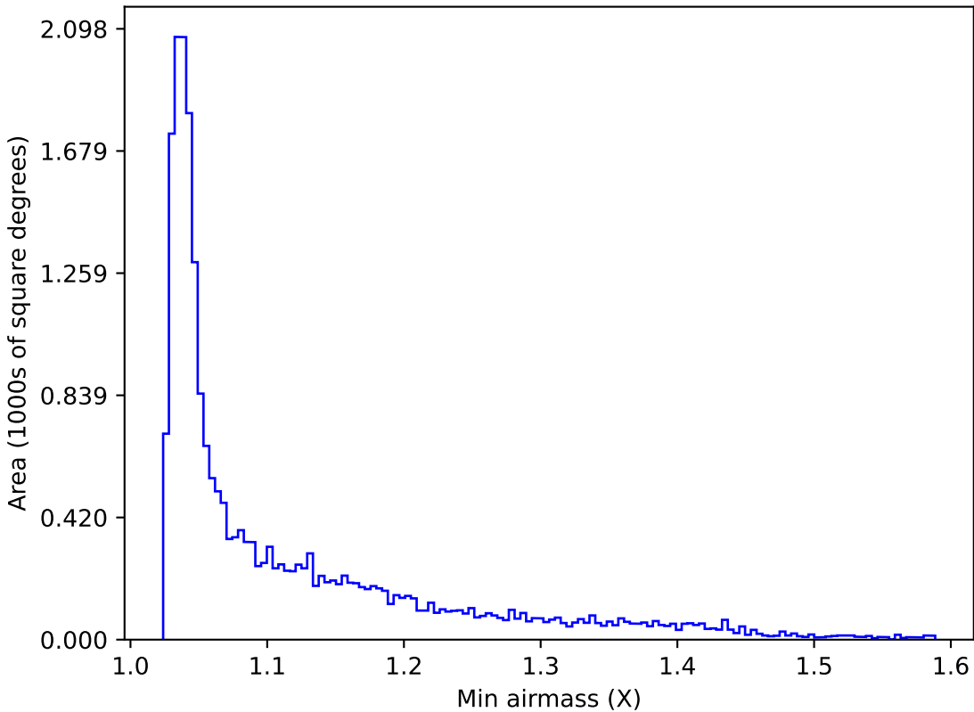
ddf_loaded_fl1_v3.4_10yrs All sky u band: Min airmass
