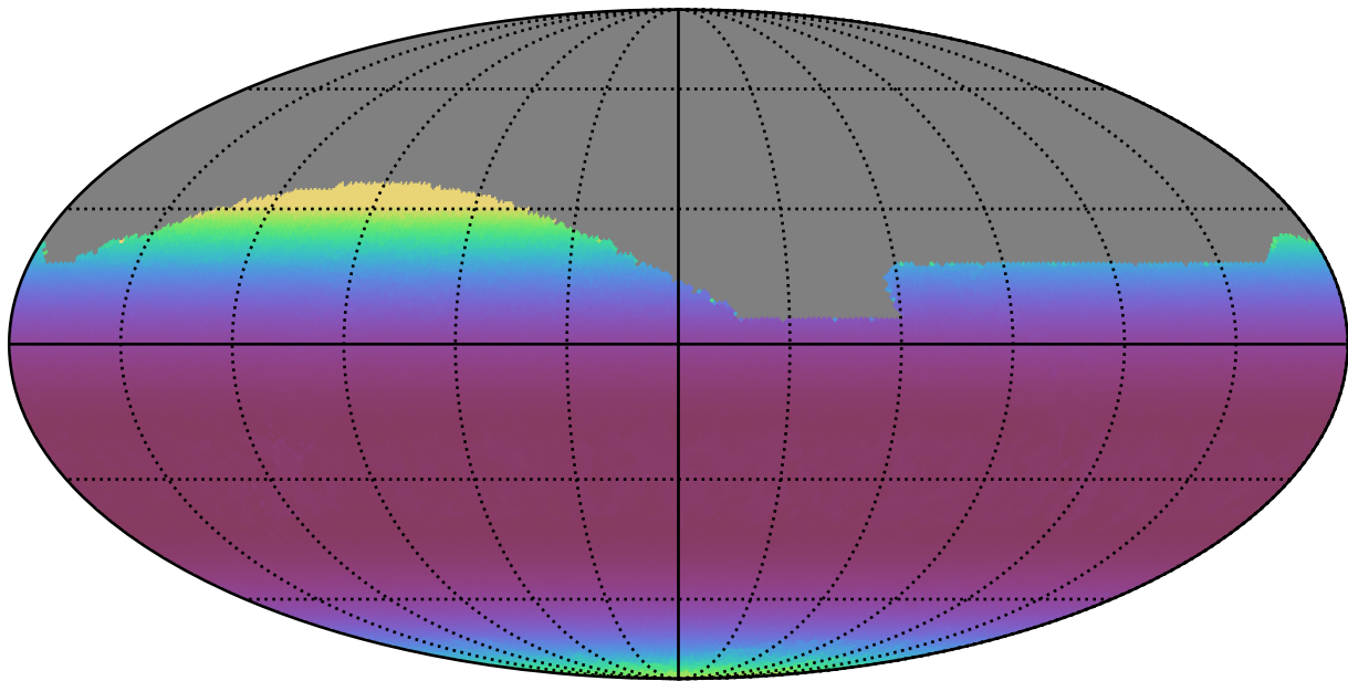
ddf_loaded_fl1_v3.4_10yrs All sky r band: Min airmass
