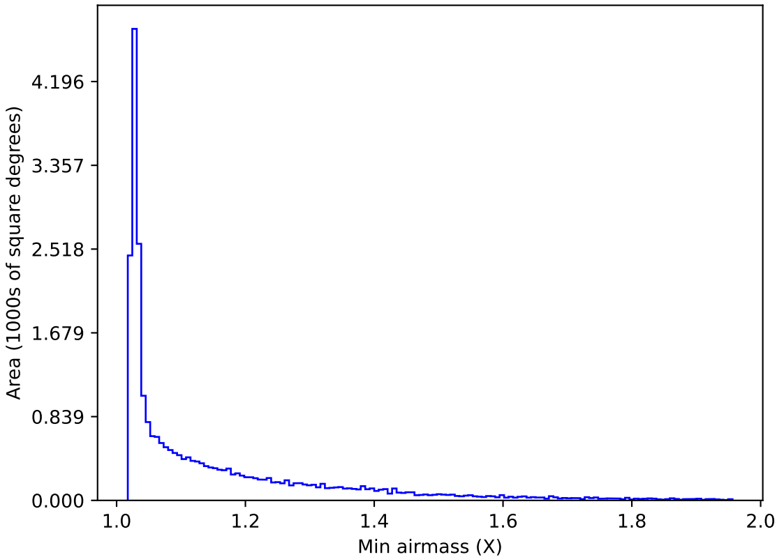
ddf_loaded_fl1_v3.4_10yrs All sky r band: Min airmass
