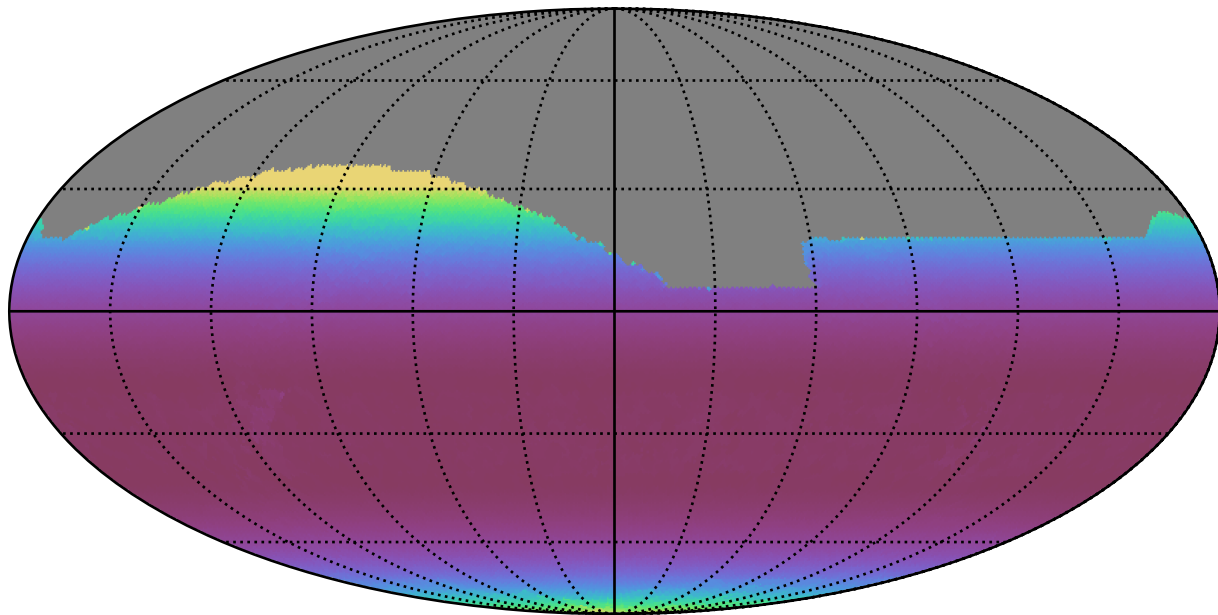
ddf_loaded_fl1_v3.4_10yrs All sky i band: Min airmass
