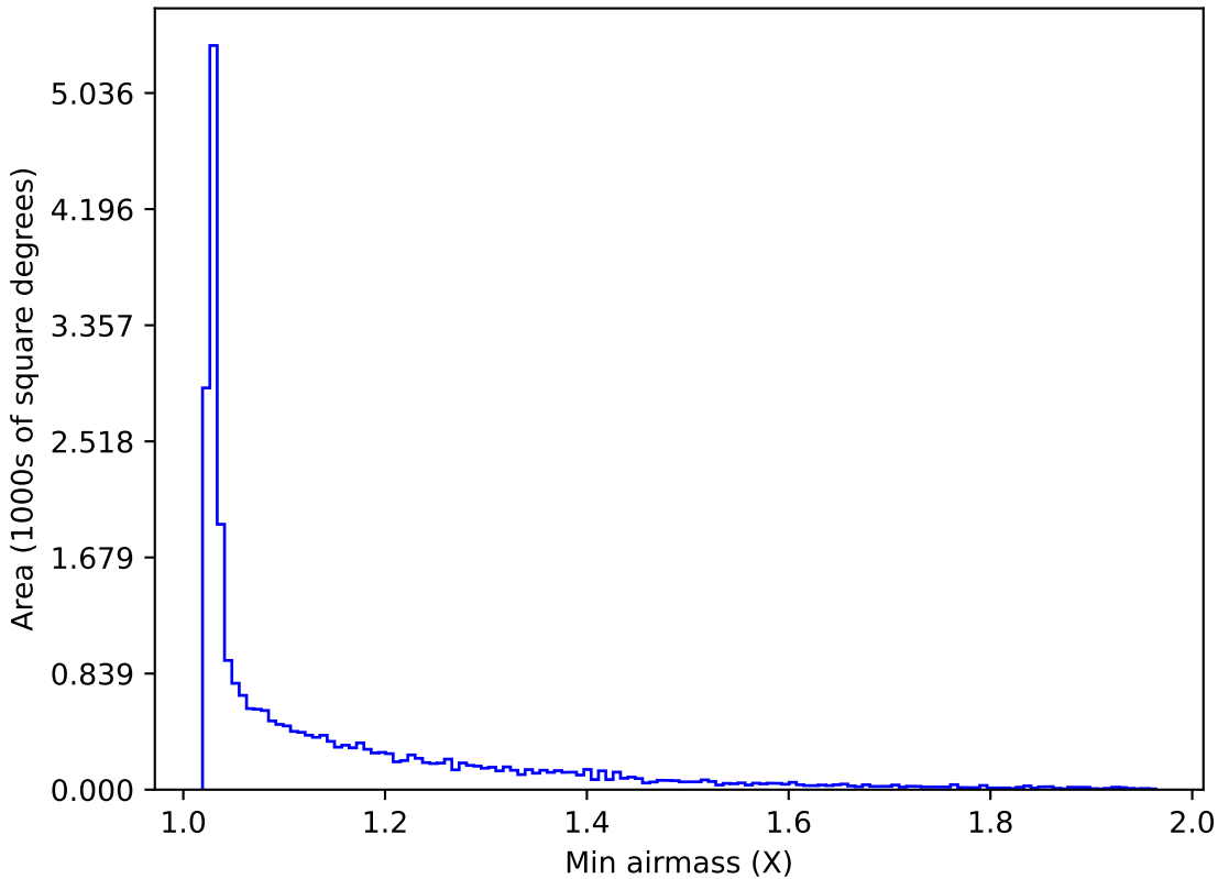
ddf_loaded_fl1_v3.4_10yrs All sky i band: Min airmass
