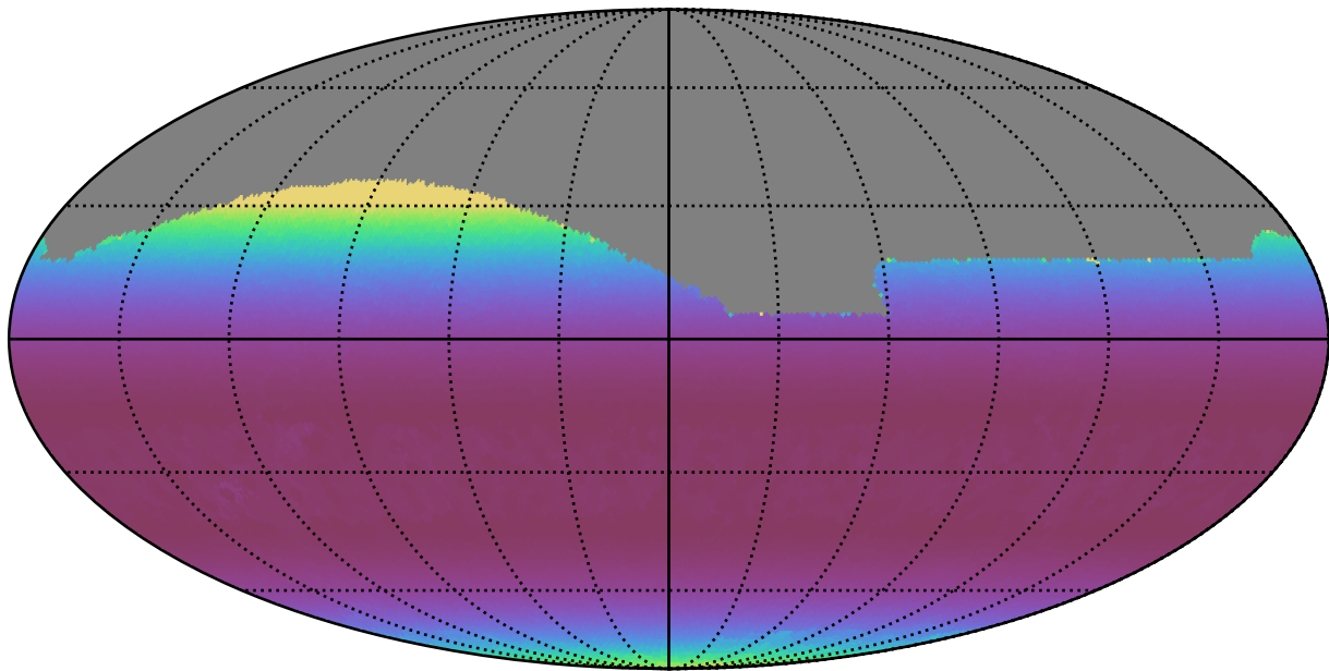
ddf_loaded_fl1_v3.4_10yrs All sky g band: Min airmass
