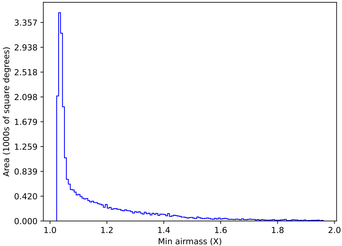
ddf_loaded_fl1_v3.4_10yrs All sky g band: Min airmass
