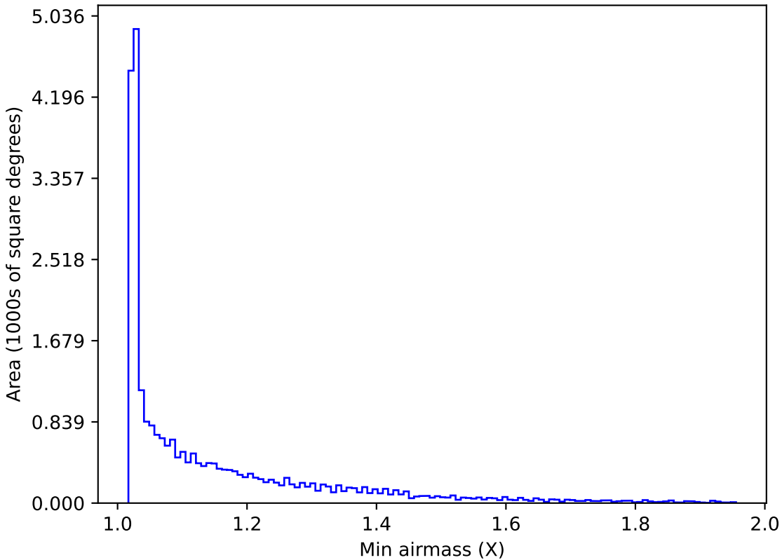
ddf_loaded_fl1_v3.4_10yrs All sky all bands: Min airmass
