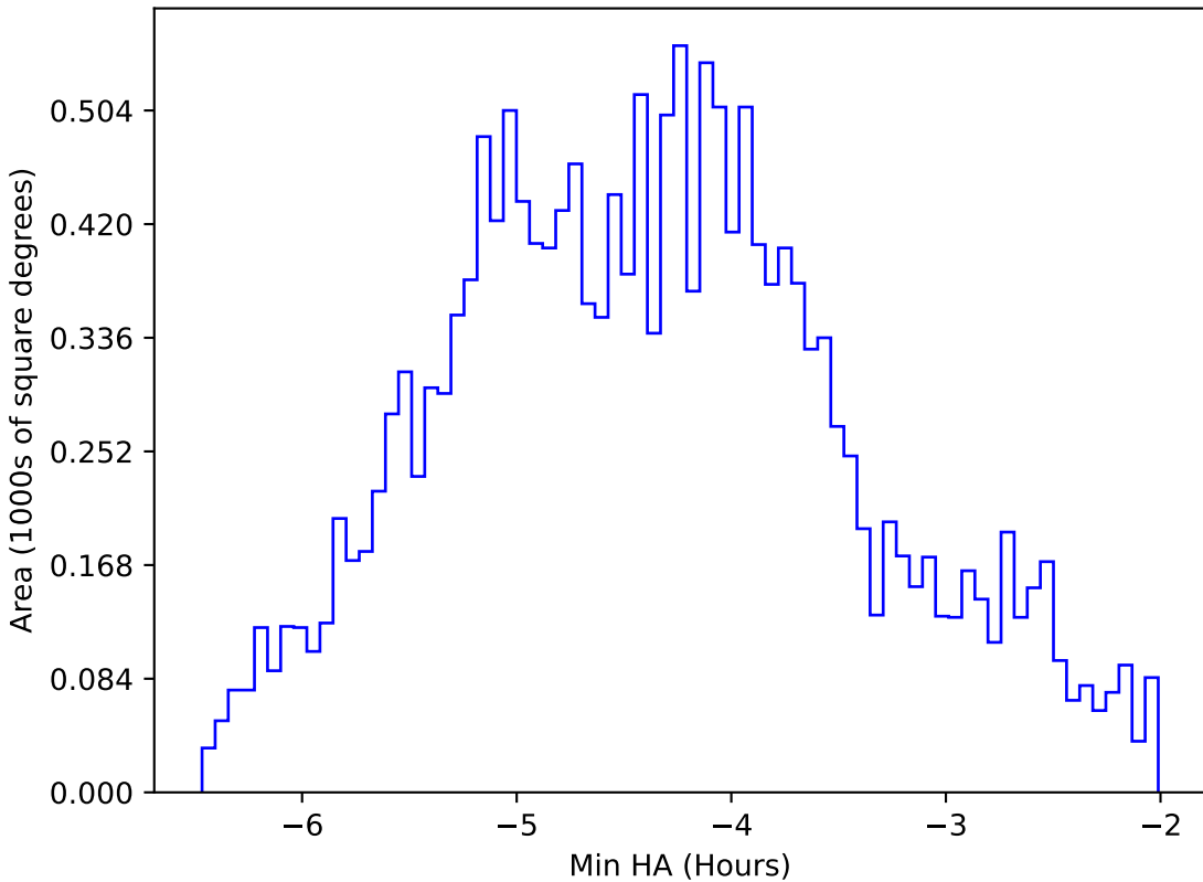
ddf_loaded_fl1_v3.4_10yrs WFD z band: Min HA
