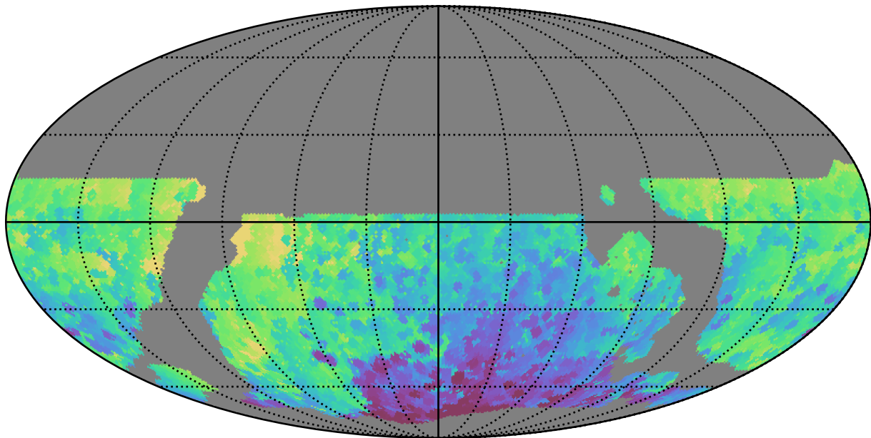
ddf_loaded_fl1_v3.4_10yrs WFD y band: Min HA
