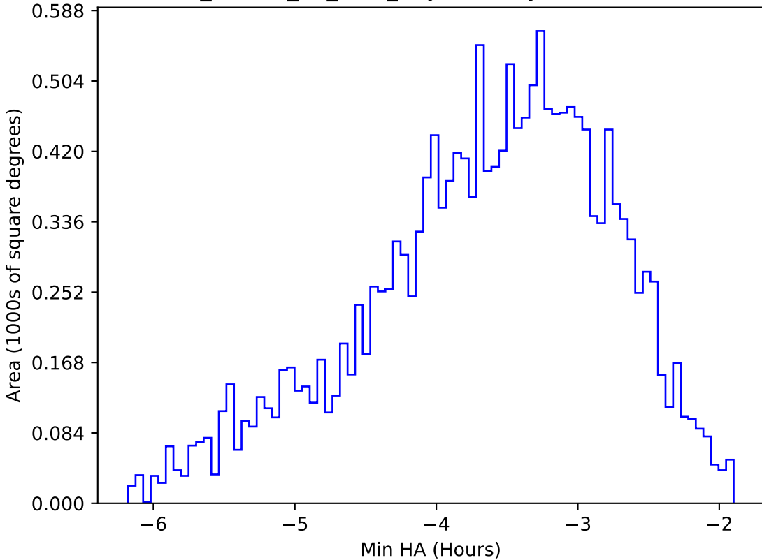
ddf_loaded_fl1_v3.4_10yrs WFD y band: Min HA
