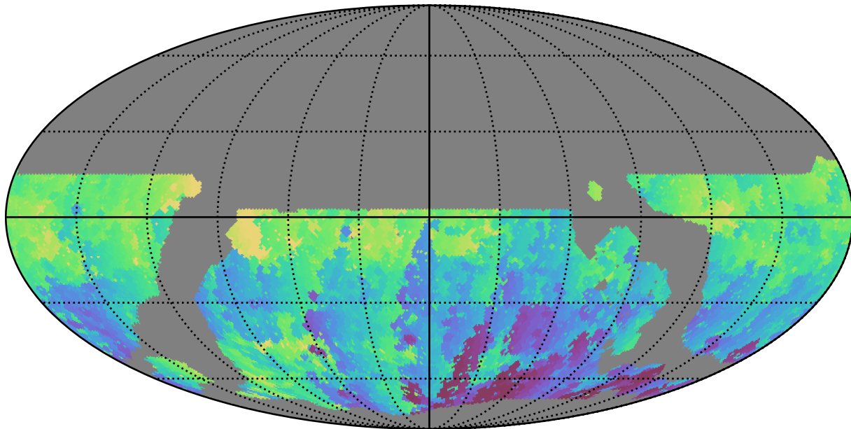
ddf_loaded_fl1_v3.4_10yrs WFD u band: Min HA
