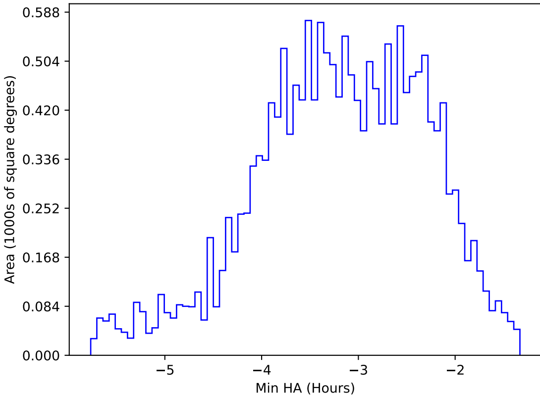
ddf_loaded_fl1_v3.4_10yrs WFD u band: Min HA
