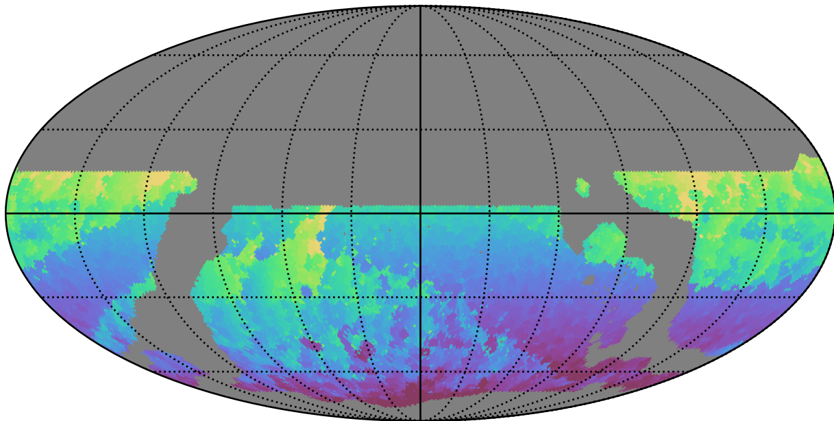
ddf_loaded_fl1_v3.4_10yrs WFD r band: Min HA
