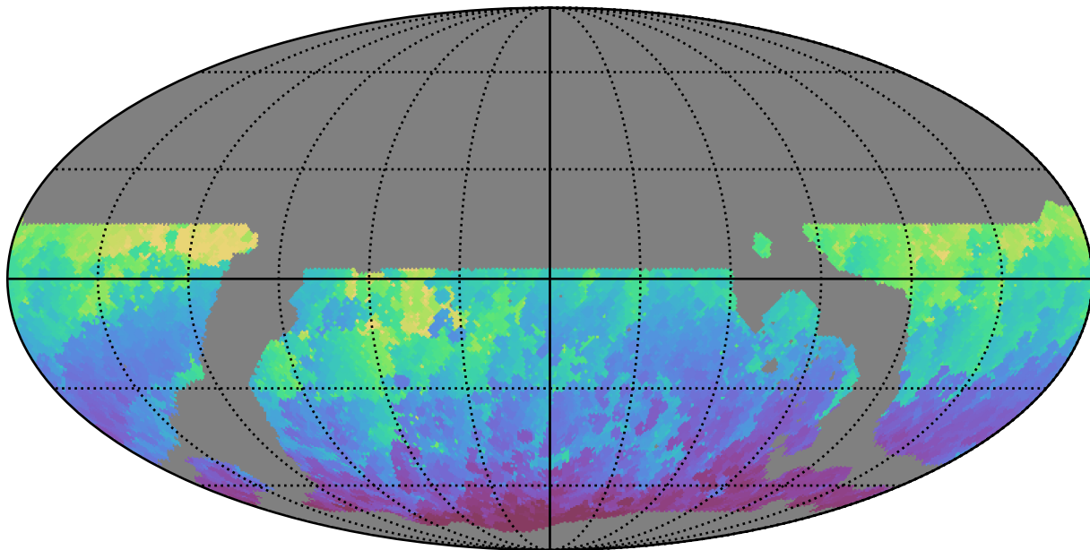
ddf_loaded_fl1_v3.4_10yrs WFD i band: Min HA
