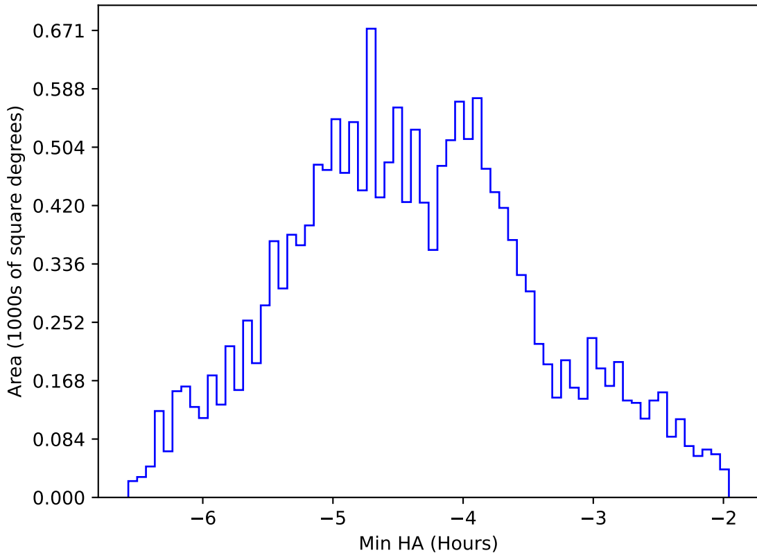
ddf_loaded_fl1_v3.4_10yrs WFD i band: Min HA
