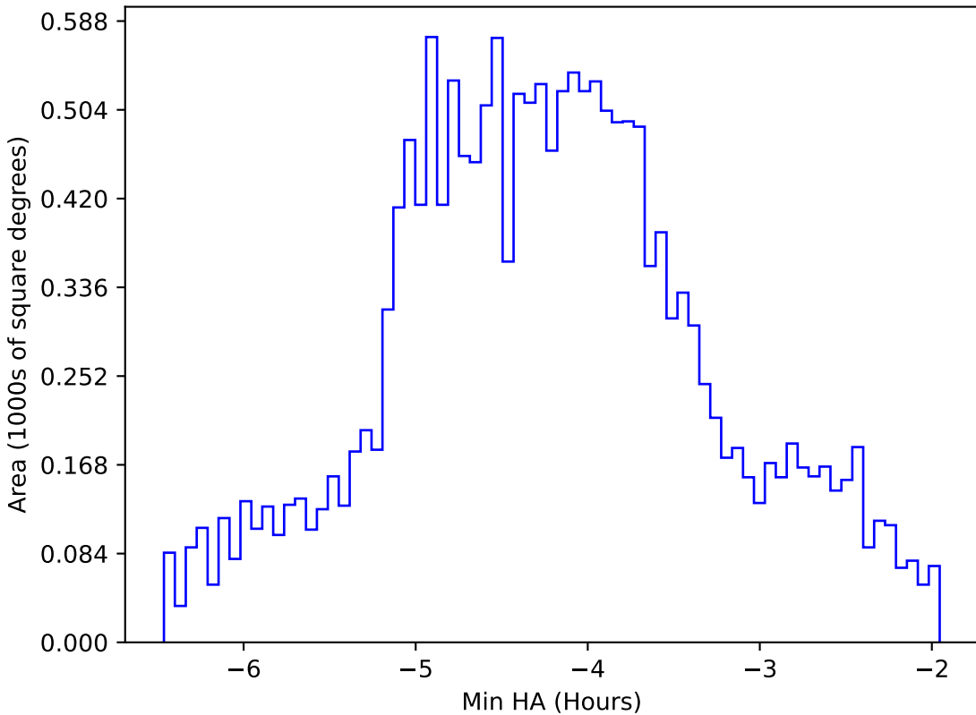
ddf_loaded_fl1_v3.4_10yrs WFD g band: Min HA
