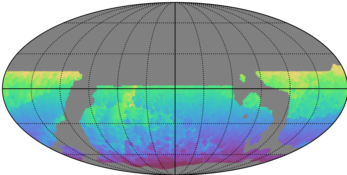
ddf_loaded_fl1_v3.4_10yrs WFD all bands: Min HA
