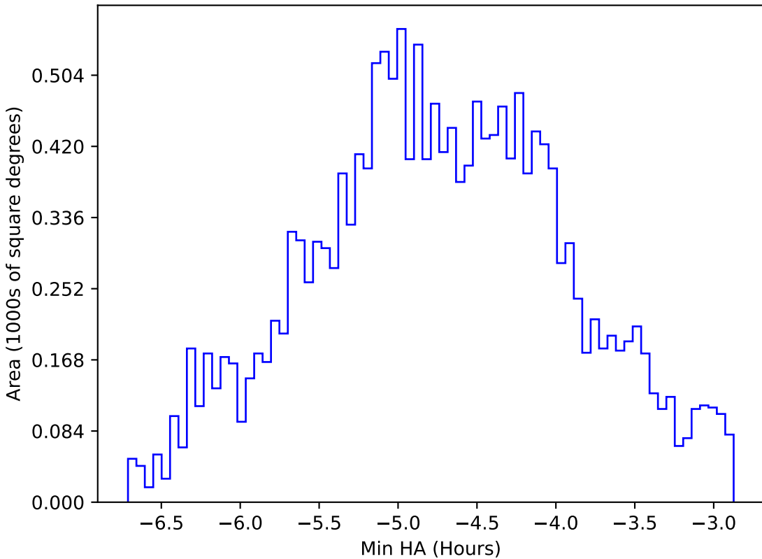
ddf_loaded_fl1_v3.4_10yrs WFD all bands: Min HA
