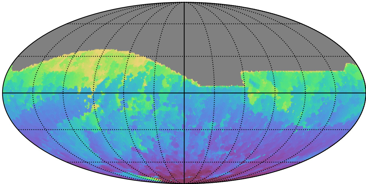
ddf_loaded_fl1_v3.4_10yrs All sky z band: Min HA
