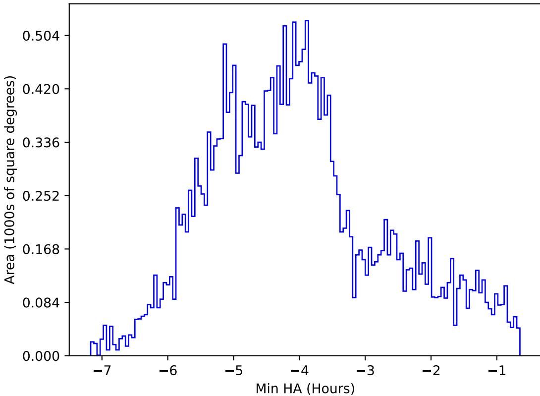
ddf_loaded_fl1_v3.4_10yrs All sky z band: Min HA
