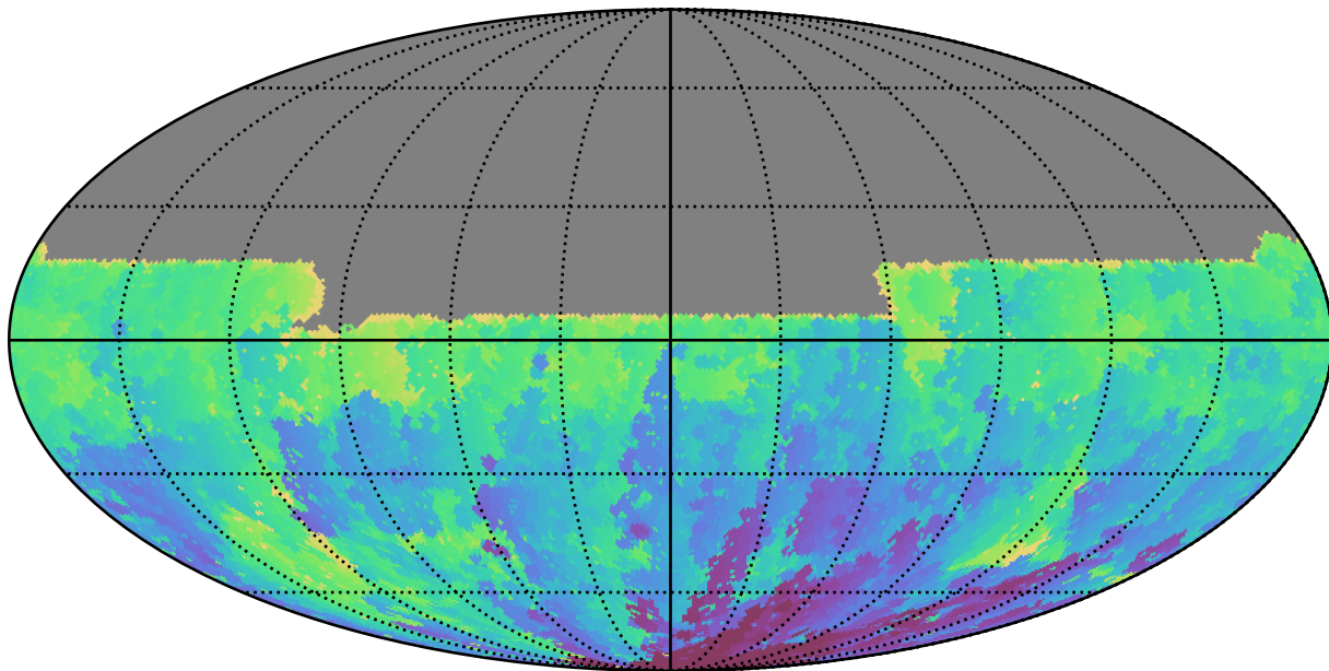
ddf_loaded_fl1_v3.4_10yrs All sky u band: Min HA
