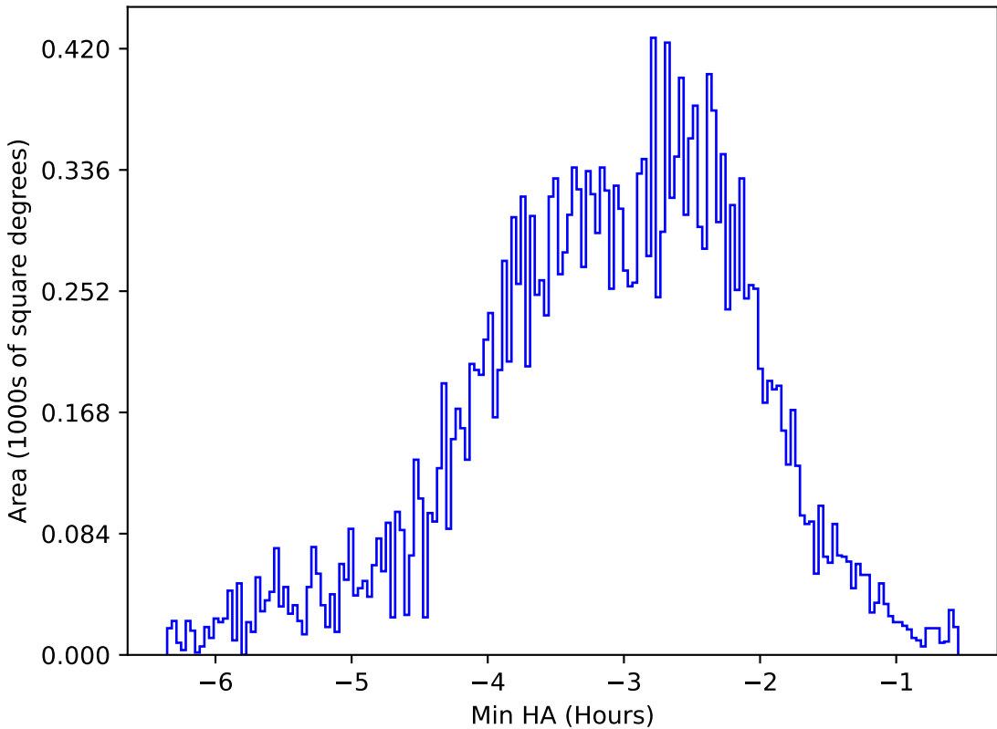
ddf_loaded_fl1_v3.4_10yrs All sky u band: Min HA
