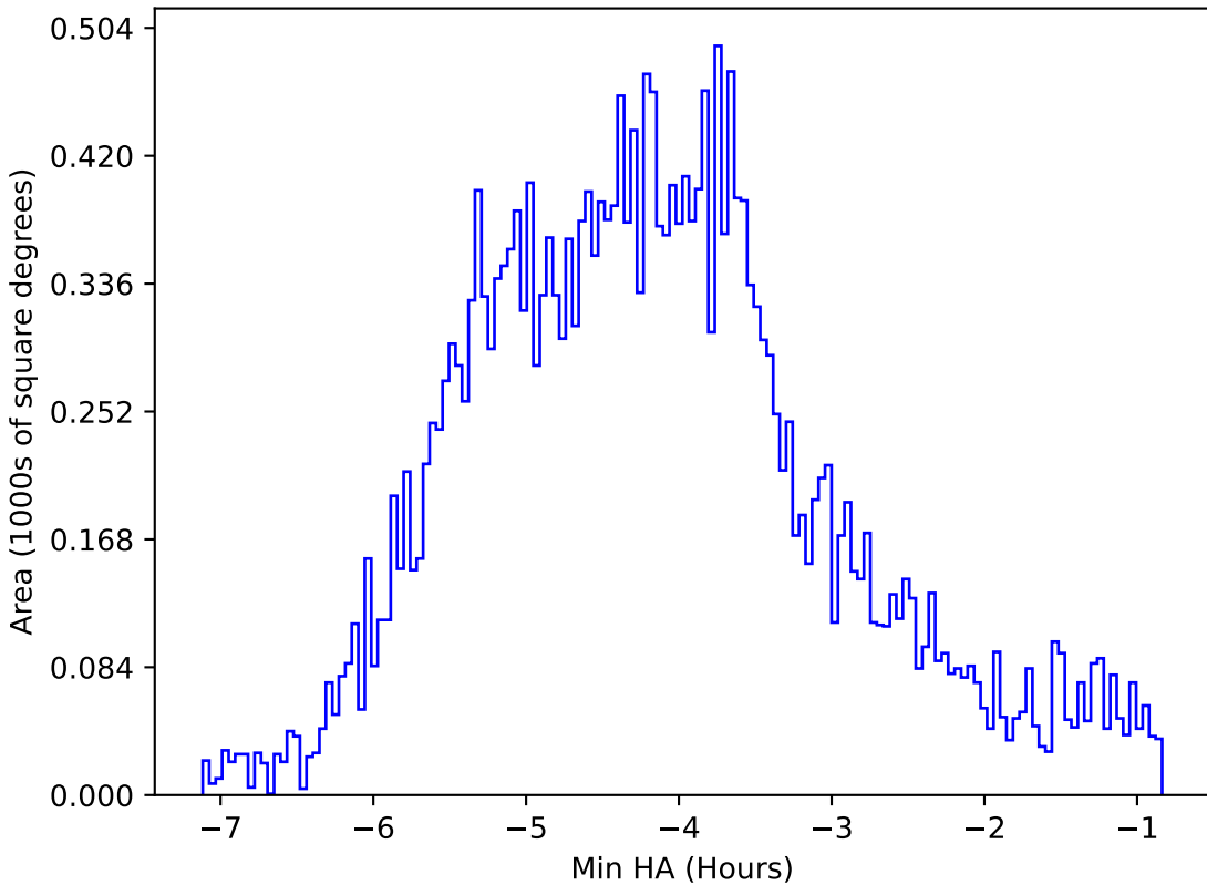
ddf_loaded_fl1_v3.4_10yrs All sky r band: Min HA
