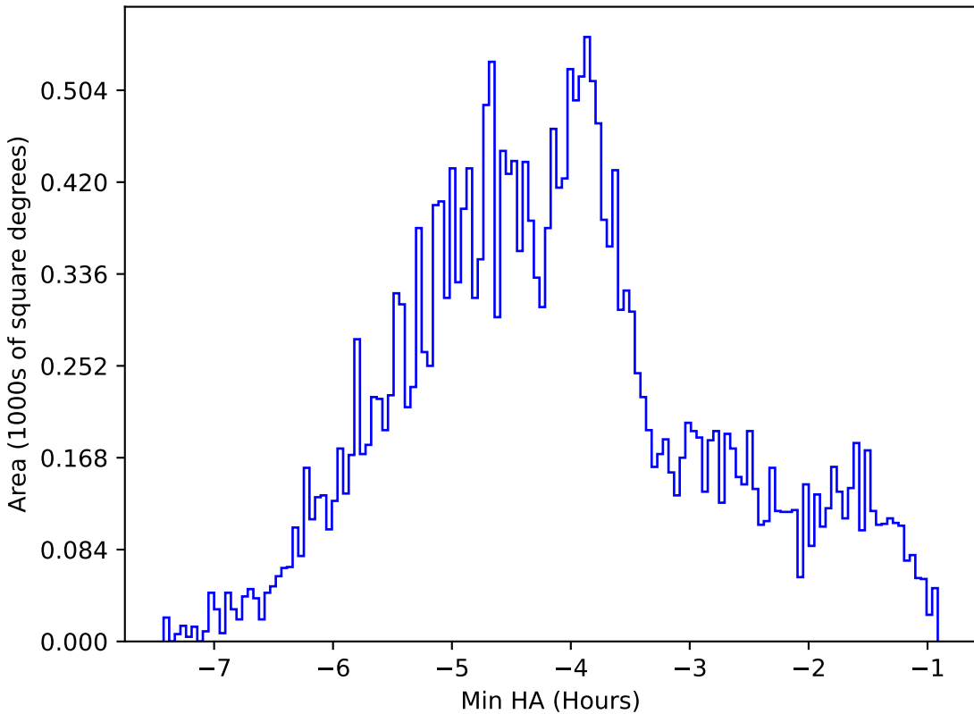
ddf_loaded_fl1_v3.4_10yrs All sky i band: Min HA
