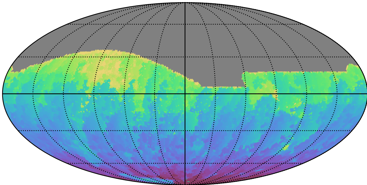
ddf_loaded_fl1_v3.4_10yrs All sky g band: Min HA
