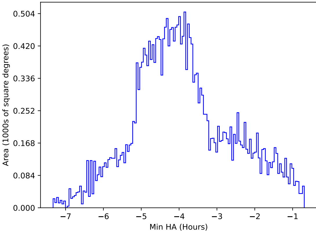
ddf_loaded_fl1_v3.4_10yrs All sky g band: Min HA
